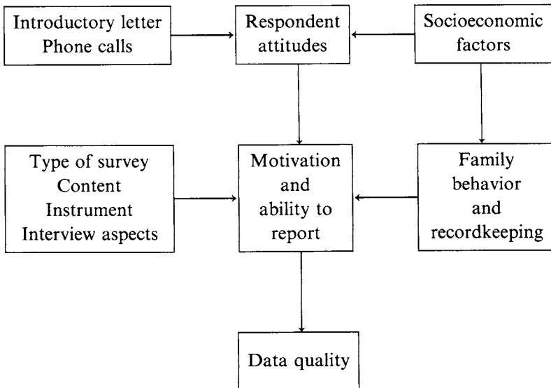
Fig. 1. Response process
